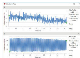
Time Waveform
