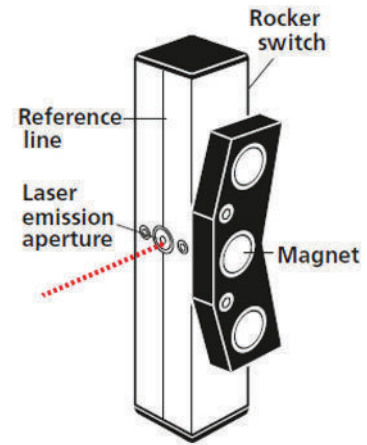
Laser unit
